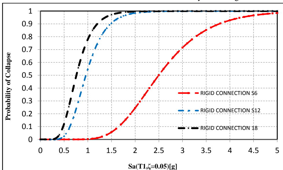
Fig 8. Collapse fragility curves of 6-, 12- and 18-stories frame considering IM=Sa(T_1, \xi = 0.05) and rigid connections
