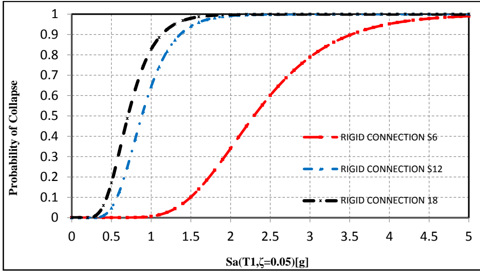
Fig 9. Collapse fragility curves of 6-, 12- and 18-stories frame considering IM=Sa(T_1, \zeta = 0.05) and semi-rigid connections (70% rigidity percentage)
