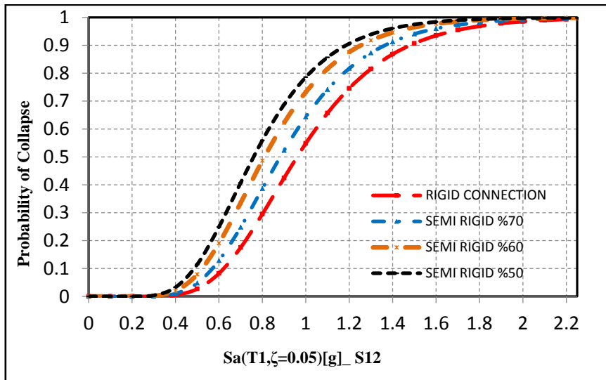
Fig 6. Collapse fragility curves of 12-story frame considering IM=Sa (T_1, \xi = 0.05)
