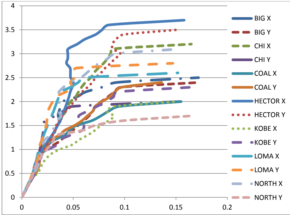
Fig 4. IDA curve of 6-story of 2-D frame with the rigid connections
