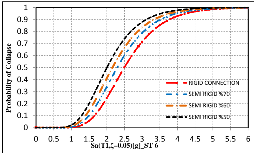
Fig 5.Collaps fragility curves of 6-story frame considering IM=Sa (T_1, \xi = 0.05)
