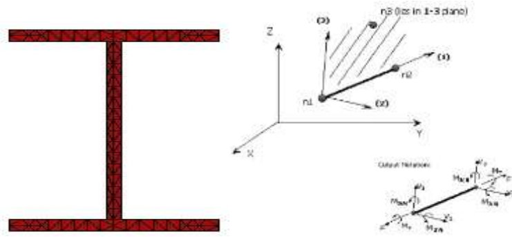
Fig 2. Geometric properties of the element [16]
