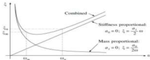
Fig 3. Relation between damping ratio and frequency for Rayleigh damping [17]
