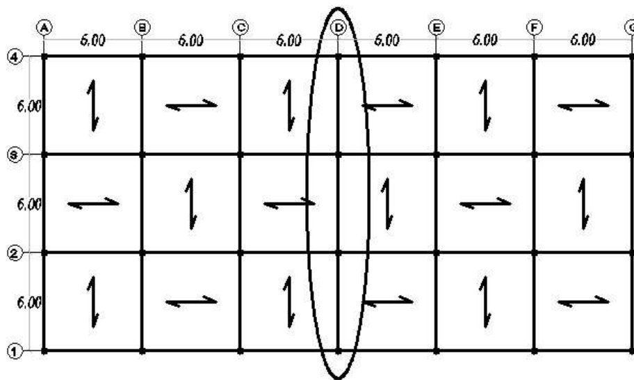
Fig.1. Frame plan of the studied building
