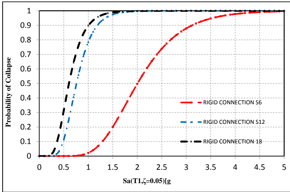
Fig 11. Collapse fragility curves of 6-, 12- and 18-stories frame considering IM=Sa (T_1, \xi = 0.05) and semi-rigid connections (50% rigidity percentage)
