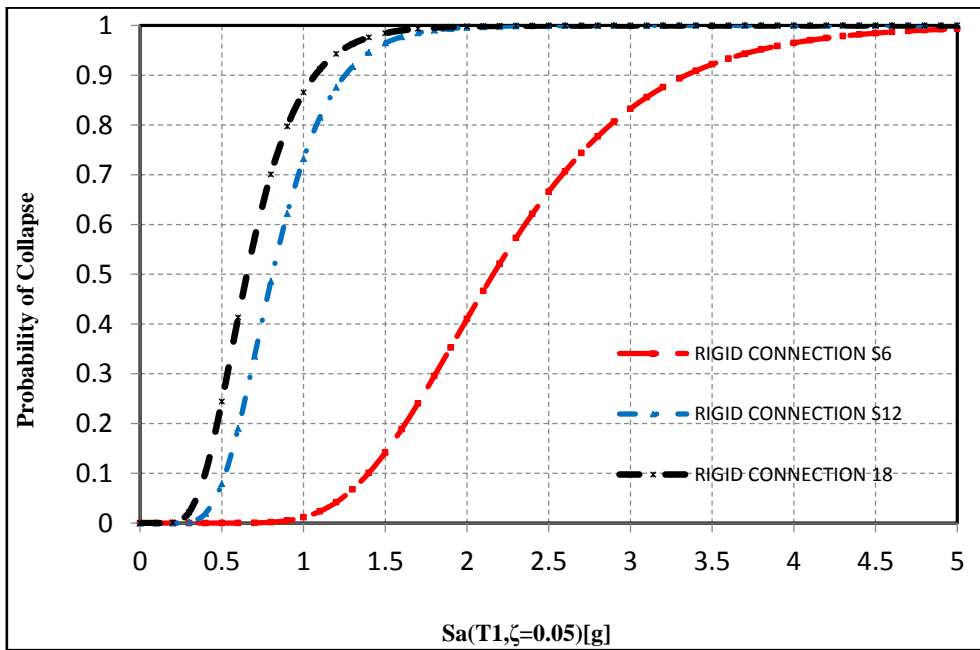
Fig 10. Collapse fragility curves of 6-, 12- and 18-stories frame considering IM=Sa(T_1, \zeta = 0.05) and semi-rigid connections (60% rigidity percentage)
