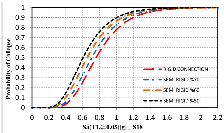
Fig 7.collaps Fragility curves of 18-story frame with IM=Sa (T_1, \xi = 0.05)
